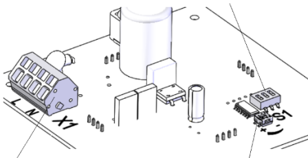
X1 Operating voltage connection S1 Light intensity control (15 – 100%)
