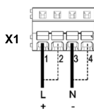
X1 External control input X2 Operating mode selection S1 Light intensity control (15 -100%)
